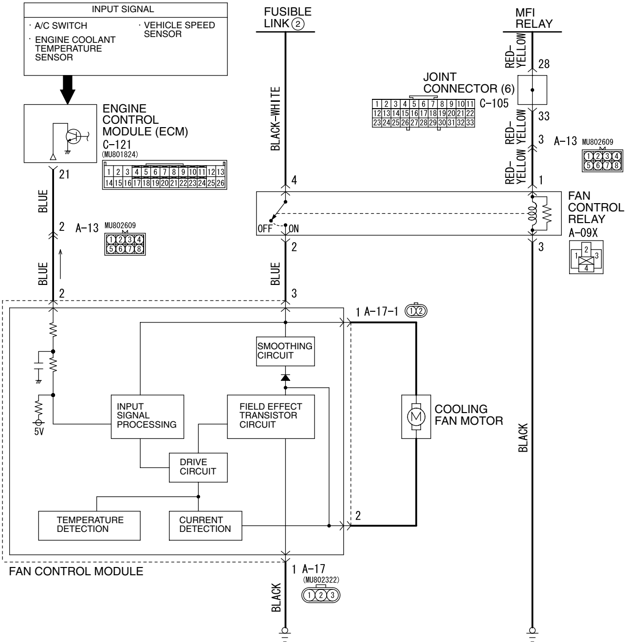
Cooling Fan Drive Circuit
